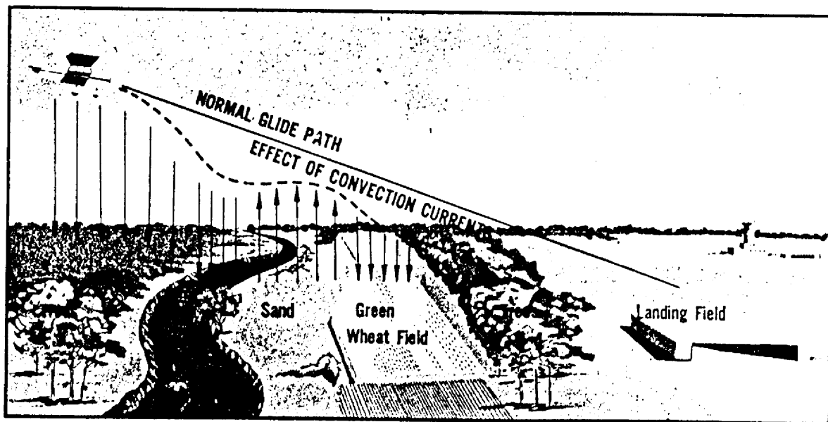
FIGURE 76. Effect of convective currents on final approach. Predominantly upward currents (top) tend to cause the aircraft to overshoot. Predominantly downward currents (bottom) tend to cause the craft to undershoot.
