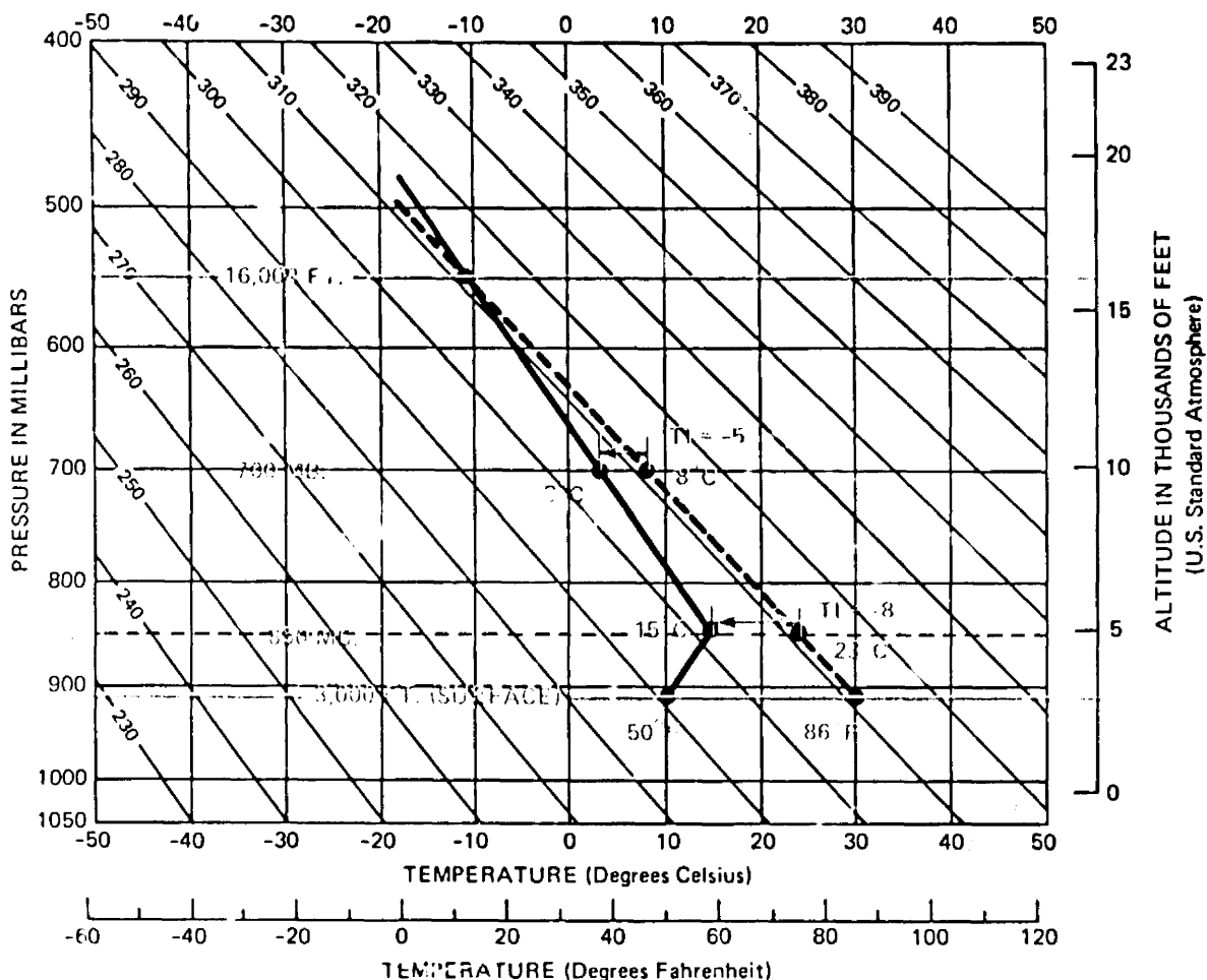
FIGURE 163. Another example of computing TI 's and maximum height of thermals. See discussion in caption of figure 162. By the time of maximum heating, excellent lift should be available in lower levels and moderate lift above 10,000 feet. Although thermals should continue to 16,000 feet, you could expect weak lift above 12,000 or 13,000 feet because of the small difference between temperatures in the thermal and in the surrounding air.
