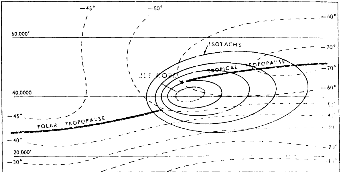
FIGURE 123. A cross section of the upper troposphere and lower stratosphere showing the tropopause and associated features. Note the "break" between the high tropical and the lower polar tropopauses. Maximum winds occur in the vicinity of this break.
