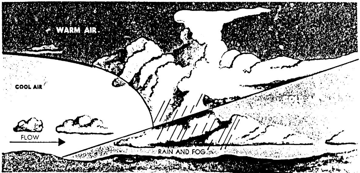
FIGURE 73. A warm front occlusion lifting warm, moist, unstable air. Note that the associated weather is complex and encompasses all types of weather associated with both the warm and cold fronts when air is moist and unstable.
