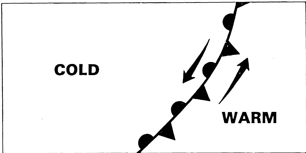
FIGURE 61. Cross section of a stationary front (top) and its weather map symbol (bottom). The symbol is a line with alternating pointed and rounded barbs on opposite sides of the line, the pointed barbs pointing away from the cold air and the rounded barbs away from the warm air. If a map is in color, the symbol is a line of alternating red and blue segments. The front has little or no movement and winds are nearly parallel to the front. The symbol in the warm air is the tail of a wind arrow into the page. The symbol in the cold air is the point of a wind arrow out of the page. Slope of the front may vary considerably depending on wind and density differences across the front.
