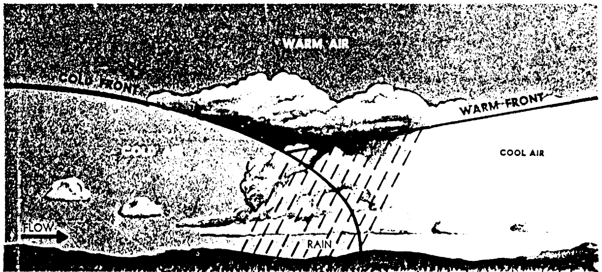
FIGURE 74. A cold front occlusion lifting warm, moist, stable air. Associated weather encompasses types of weather associated with both warm and cold fronts when air is moist and stable.
