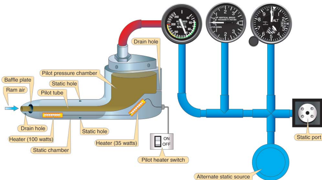
Figure 3-1. A Typical Electrically Heated Pitot-Static Head.
