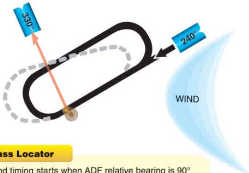
Figure 10-7. Holding—Outbound Timing.
