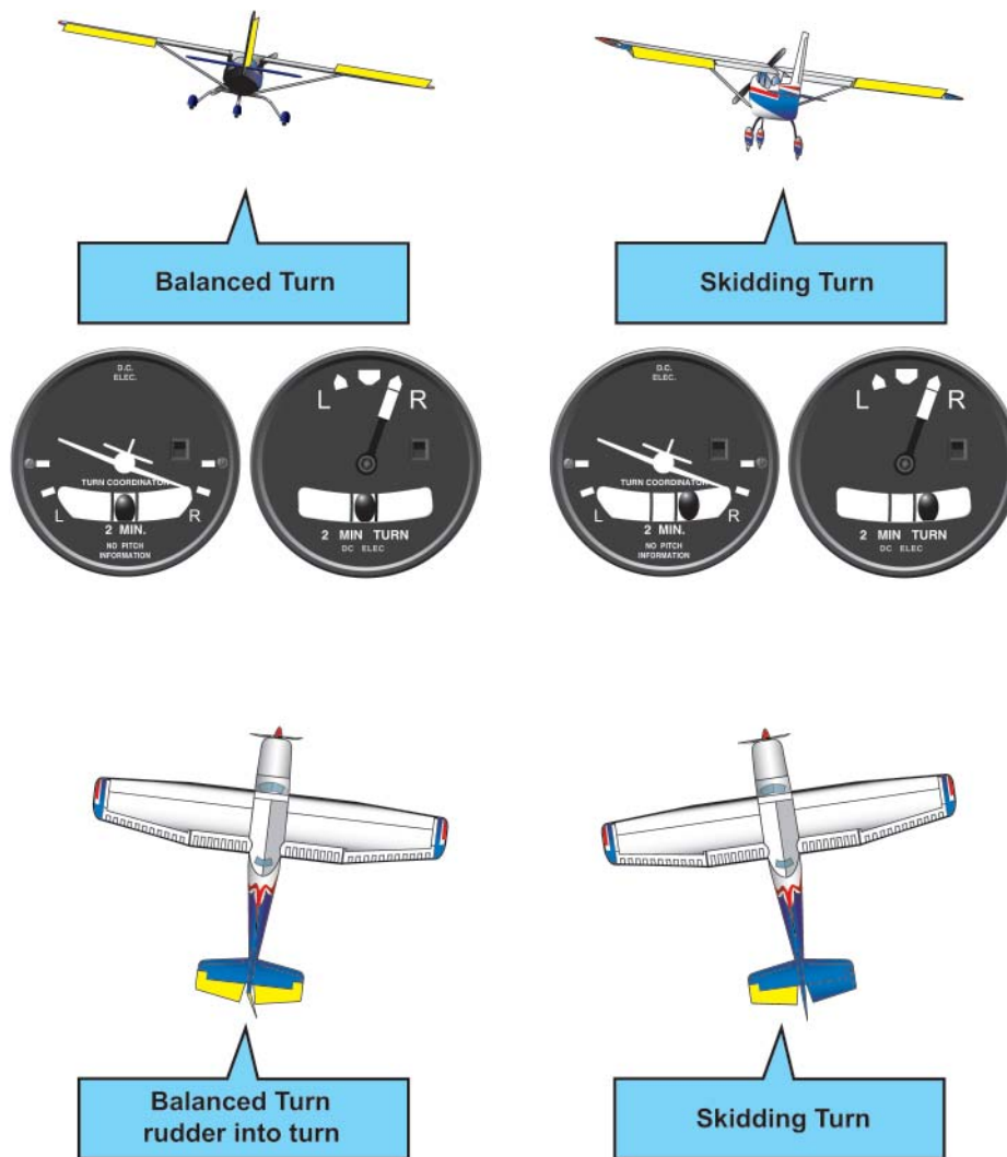
Figure 2-15. Adverse Yaw.
