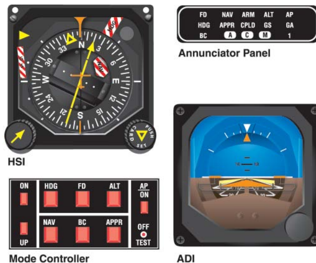
Figure 3-40. Components of a Typical Flight Director System.
