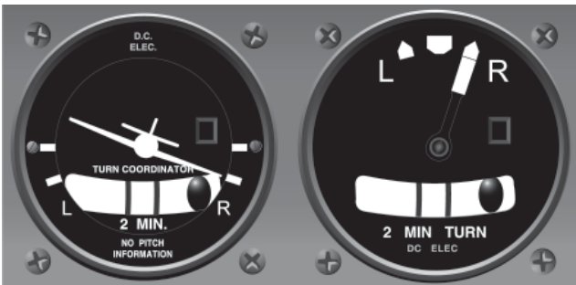
Figure 5-19. Slip Indication.
