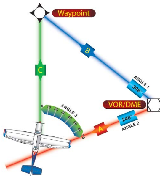
Figure 7-22. RNAV Computation.
