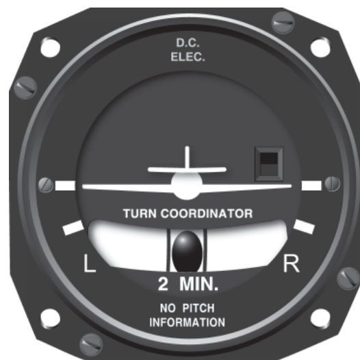
Figure 3-35. A turn coordinator senses rotation about both roll and yaw axes.
