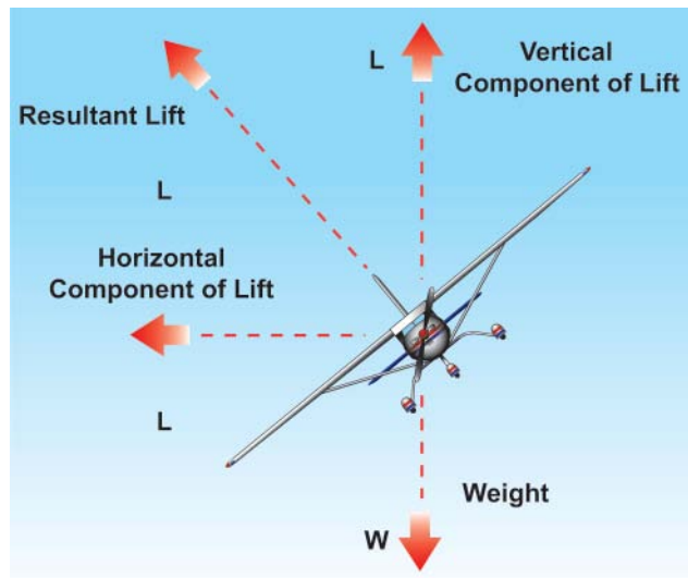
Figure 2-13. Forces In a Turn.
