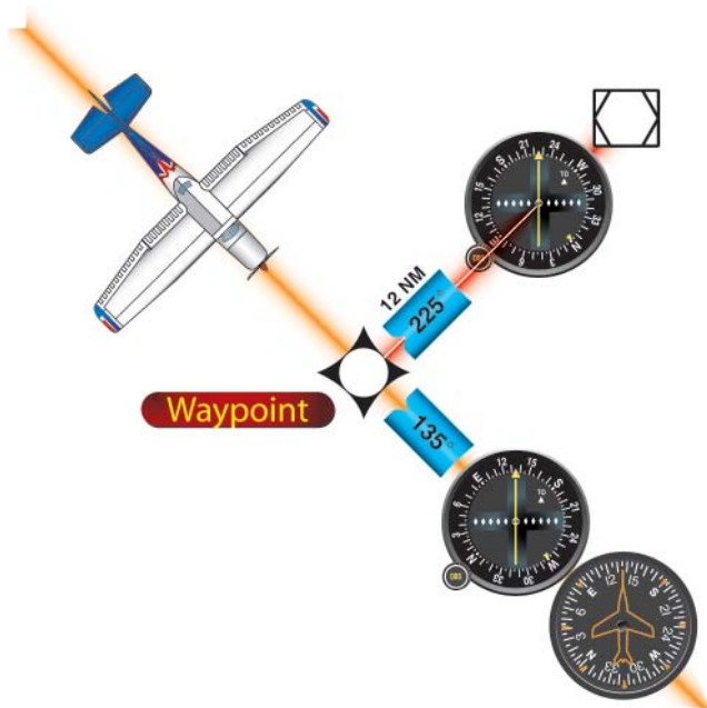
Figure 7-25. Aircraft/DME/Waypoint Relationship.
