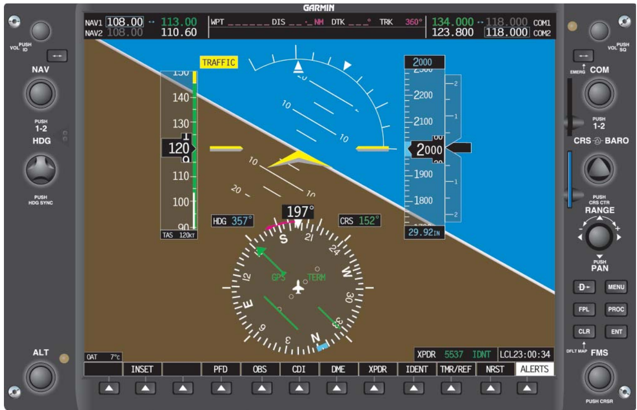
Figure 4-39. Horizontal Situation Indicator (HSI) Trend Indicator Elongates Proportionally With the Rate of Turn.
