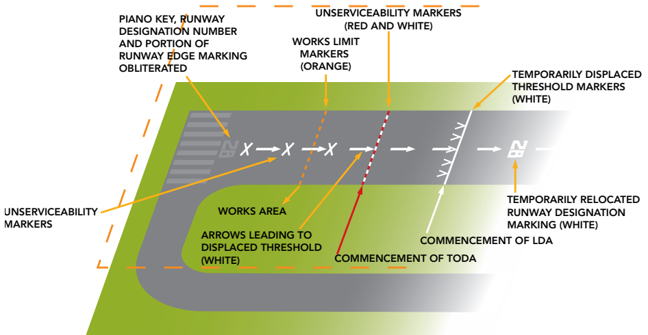
MARKINGS FOR A TEMPORARILY DISPLACED THRESHOLD DUE TO WORKS ON THE RUNWAY FOR PERIODS IN EXCESS OF 30 DAYS
